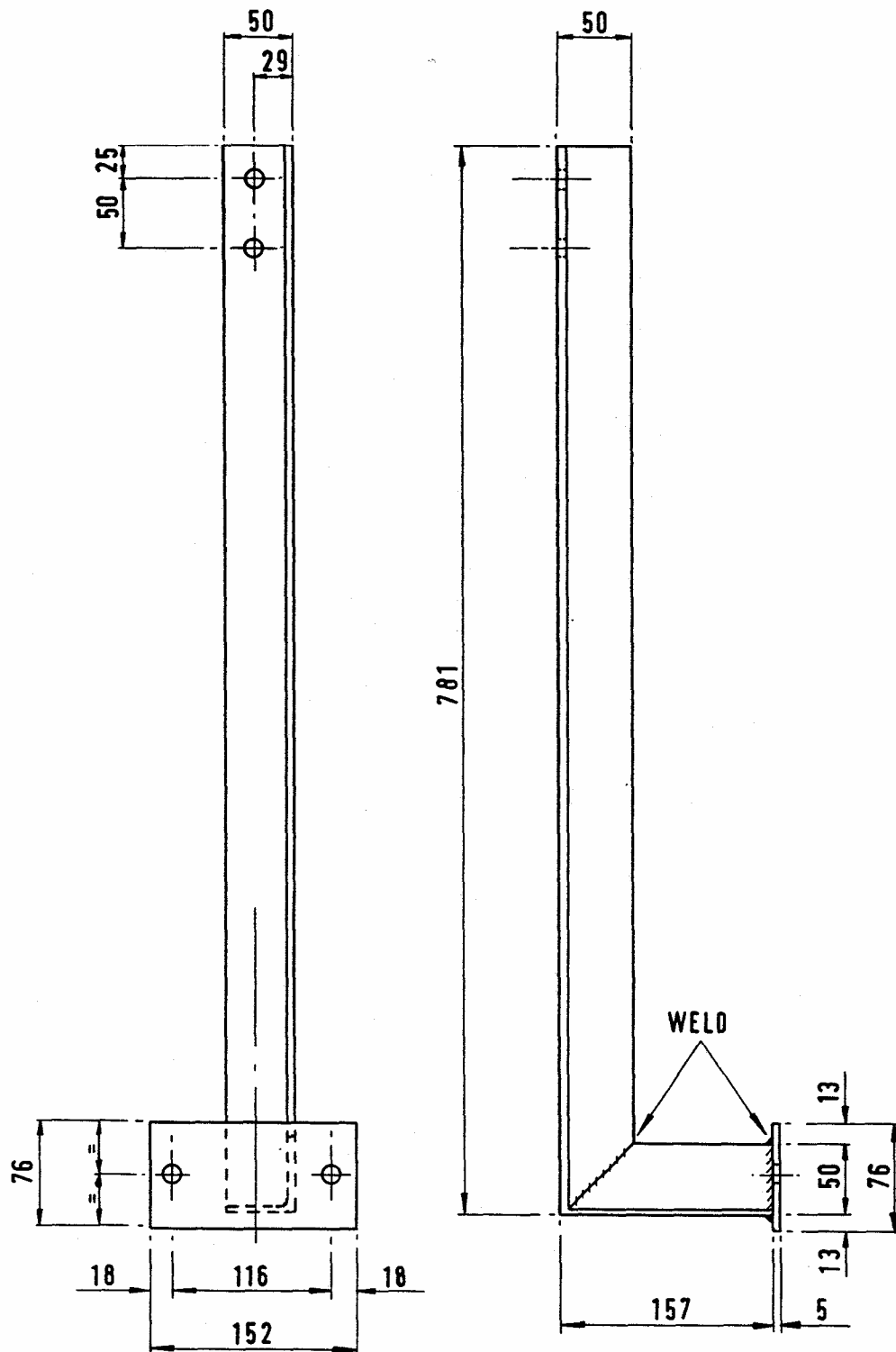
Figure 48: Cable cleat support details for 132 kV construction (ESI Drawing No. 439549)
